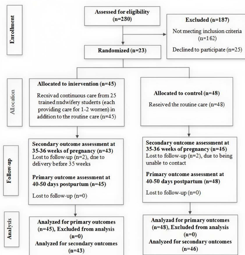
Figure 1. CONSORT Flowchart of Participant Allocation
